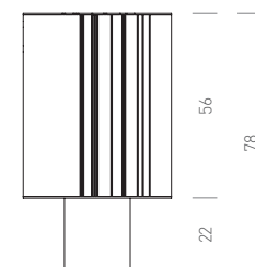
Frontal | Front view Peso | Weight: 80 kg Capacidad | Capacity: 50 L
