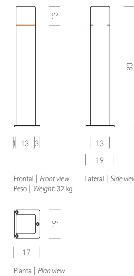
Planta | Plan view
