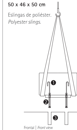
Frontal | Front view
