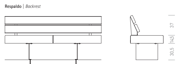
Frontal | Front view
