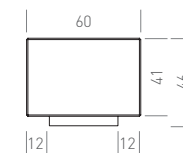
Frontal | Front view Peso | Weight: 390 kg
