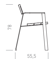
Lateral | Side view
