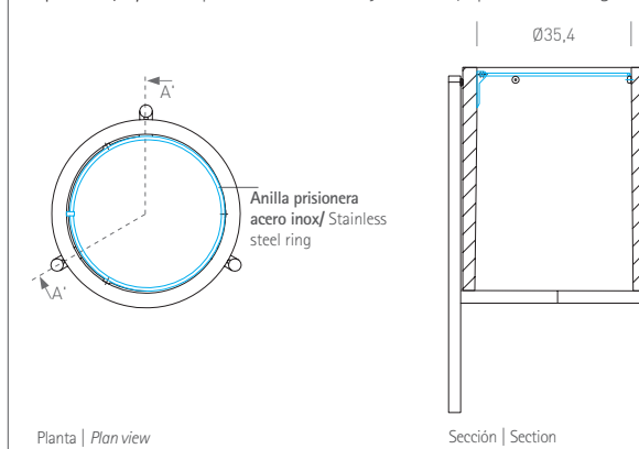
Planta | Plan view
