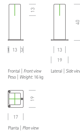
Planta | Plan view
