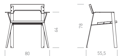
Frontal | Front view Peso | Weight: 23 kg
