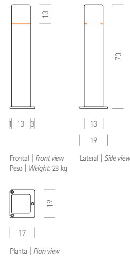
Planta | Plan view
