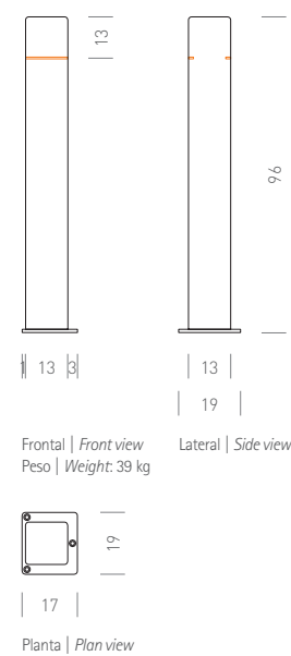
Planta | Plan view
